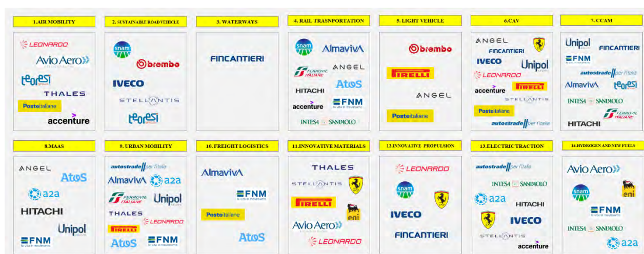
Figure B.27: tentative affiliation of companies based on their industrial business plan
